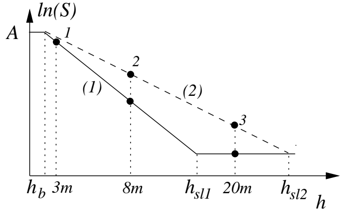
Fig. 12. Piecewise model for S(h) . Points 1, 2 and 3 correspond to the DIMMs at elevations h_1 , h_2 and h_3 . Two situations are shown. (1) the SL upper limit h_{sl1} is lower than h_3 and the 20-m DIMM is outside the SL. (2) the SL upper limit is higher than h_3 and the point 3 is inside the SL. Points 1 and 2 are supposed to be always inside the SL.
