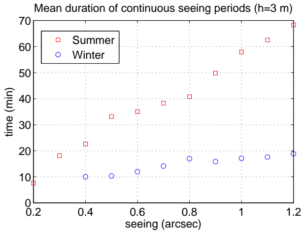
Fig. 16. Histogram of the length t_s of continuous intervals with seeing < s_0 , as a function of s_0 , for seeing data taken in summer and in winter with the DIMM at an elevation of 3 m.
