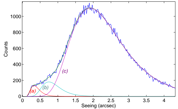
Fig. 7. Histogram of the seeing data taken by the 3-m DIMM, as usual excluding summers. As for Fig. 3, curves (a), (b), (c) represent the three log-normal fits. The mean seeing is quite poor (close to 2 arcsec), but the excellent and intermediate seeing situations are still visible, even with a telescope mount placed on the snow surface, with probabilities of about 2% and 5%.
