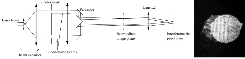
Fig. 3. Optical layout of the IRAN 2-beams laboratory experiment (left), and recorded interferometric image (fringed pupil) on the right.
