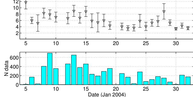
Fig. 9. Isoplanatic angle as a function of day. Top: daily median values. Error bars corresponds to the 1\sigma dispersion of the daily values. Bottom: number of data per day.
