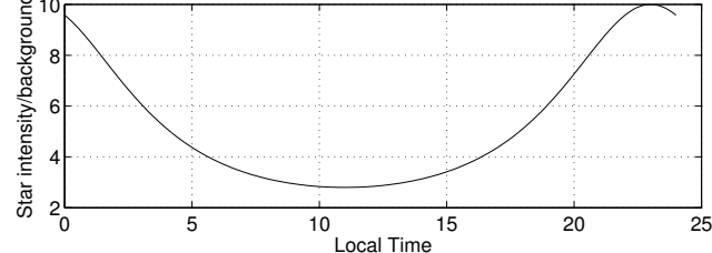
Fig. 2. Plot of the star image peak intensity I_m to the sky background level model \langle B(t) \rangle . From images taken in the period Dec 1-15, 2003.
