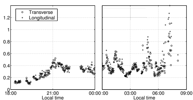
Fig. 3. First seeing curves obtained during the campaign 2003-2004 on November 21 and 22, 2003. We show here the longitudinal (+) and transverse (o) time series.
