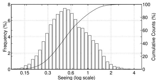
Fig. 5. Histogram (stairs) and cumulative histogram (continuous line) of seeing values for the campaigns 2003-2004 and 2004-2005. Seeing axis is in logarithmic scale.
